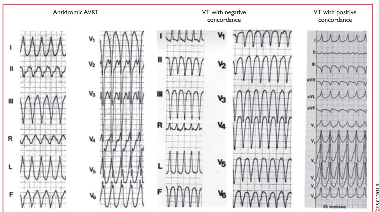
Figure 3 Examples of positive and negative chest lead concordance in VT. AVRT = atrioventricular re-entrant tachycardia; VT = ventricular tachycardia.
